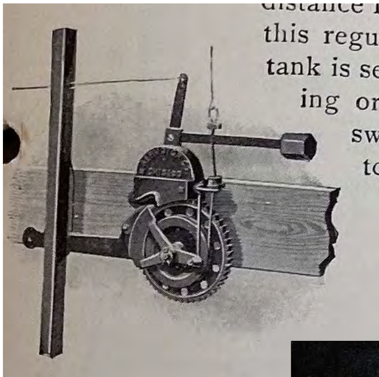
Below left: A salvaged mechanism, perhaps a regulator that controlled the float in the tank. A label cast into the casing reads: "6-8-9-10 Ft. Mills."
