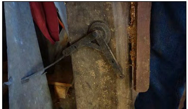
Left: The wood furl handle on the windmill at Vincent Maefsky's farm. Below: Items salvaged from the Scandia barn that might have been associated with the mill's furling mechanism or float..
