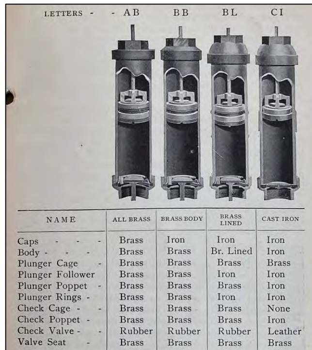
Top: Diagram of pumping cylinder (Baker, Field Guide, 19)
