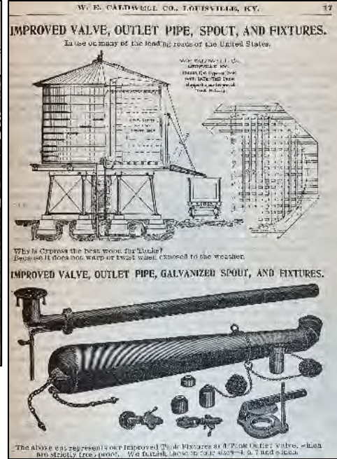
Top right: Tank with spout from catalog of W. E. Caldwell Company, 1906 (Tanks, Towers, and Tubs, 17, Northwest Architectural Archives, University of Minnesota)
